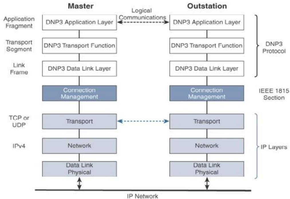
Figure 2.18: Protocol Stack for Transporting Serial DNP3 SCADA over IP
